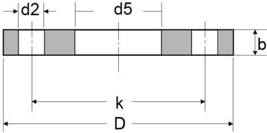
DIN 2573 PN6 PLATE FLANGE DIMENSIONS DIMENSIONS AND APPROX. FLANGE WEIGHT
