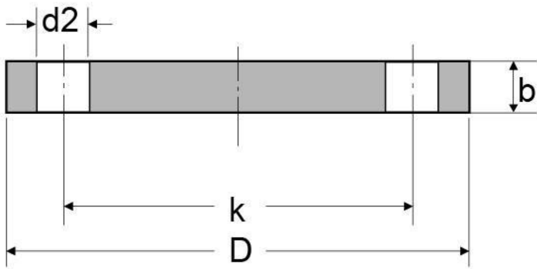
DIN 2527 PN64 BLIND FLANGE DIMENSIONS AND APPROX. FLANGE WEIGHT
