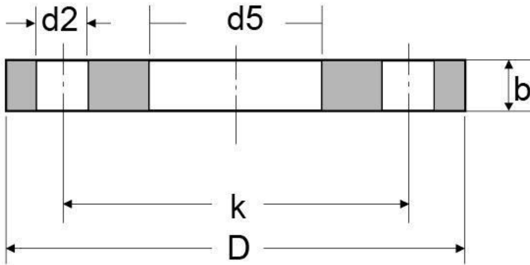
DIN 2503 PN40 PLATE FLANGE DIMENSIONS DIMENSIONS AND APPROX. FLANGE WEIGHT
