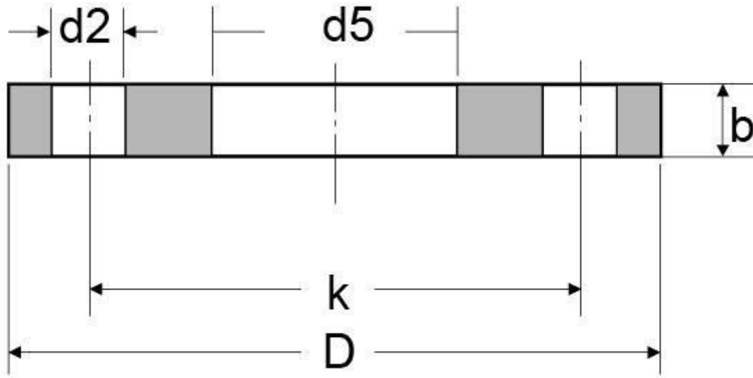
DIN 2502 PN16 PLATE FLANGE DIMENSIONS DIMENSIONS AND APPROX. FLANGE WEIGHT
